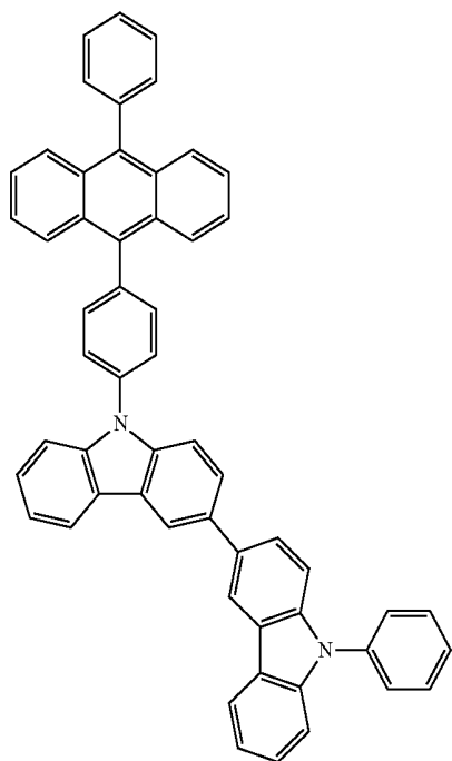
Step 1: Synthesis of 9-phenyl-3,3'-bi(9H-carbazole)] (PCC)
